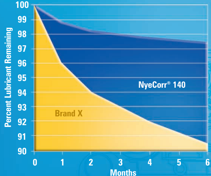
Percent Retained Oil @ 400°F
